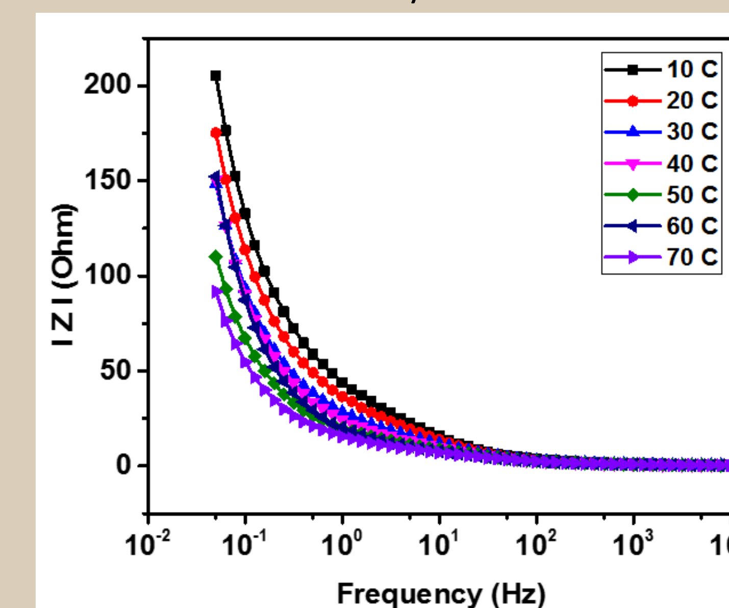
Variation of impedance as a function of frequency and temperature.
