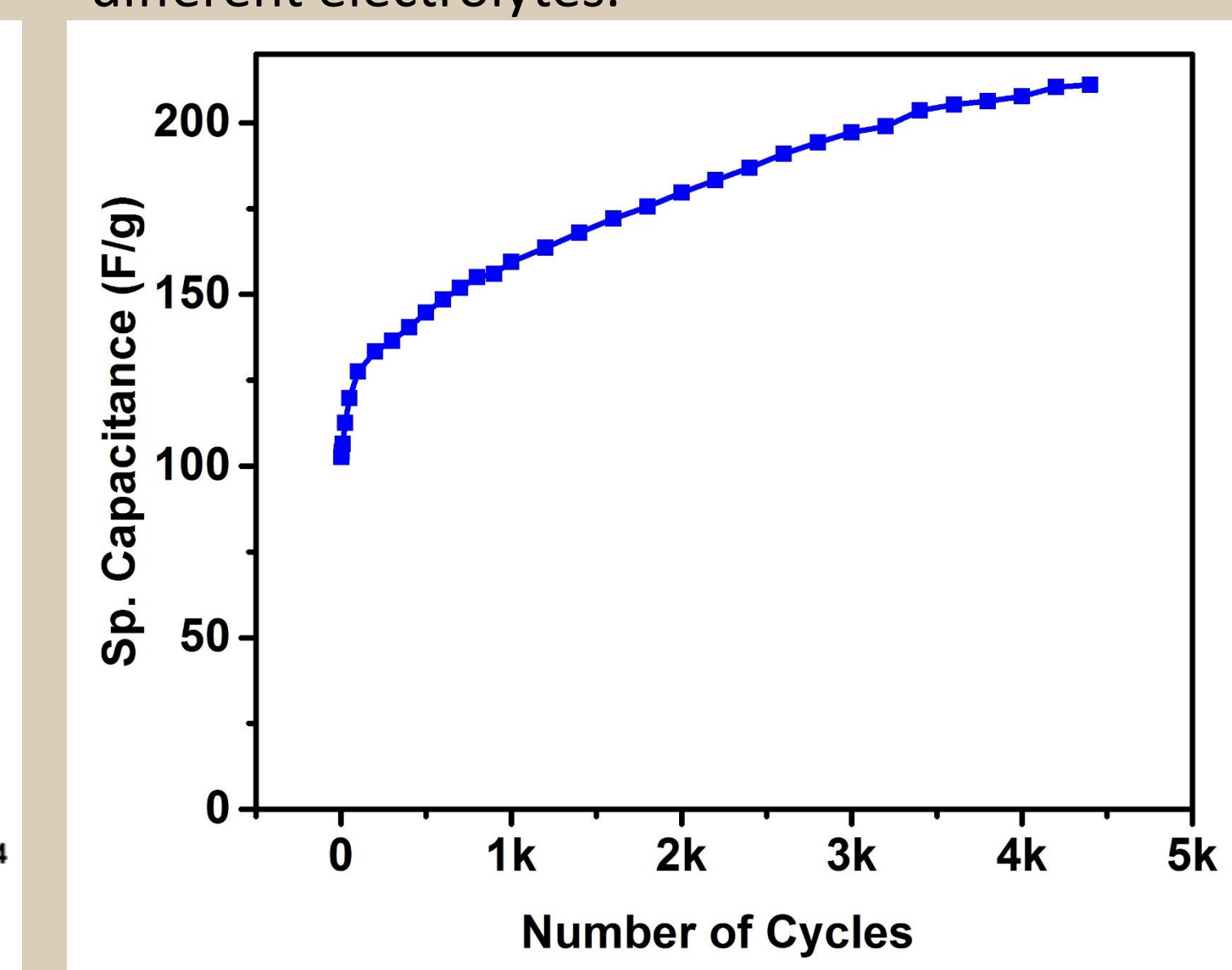
Stability test for the CMO-B sample in 3M NaOH electrolyte
