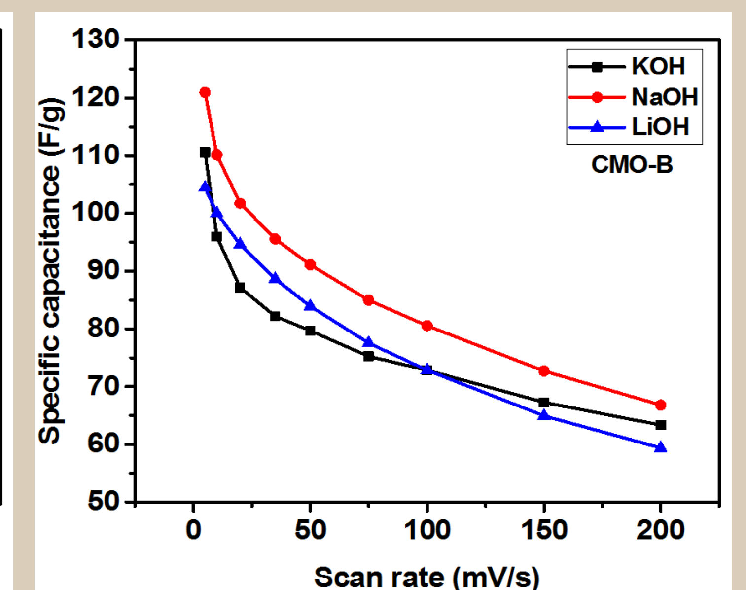
Variation of specific capacitance as a function of scan rate for CMO-B sample in different electrolytes.
