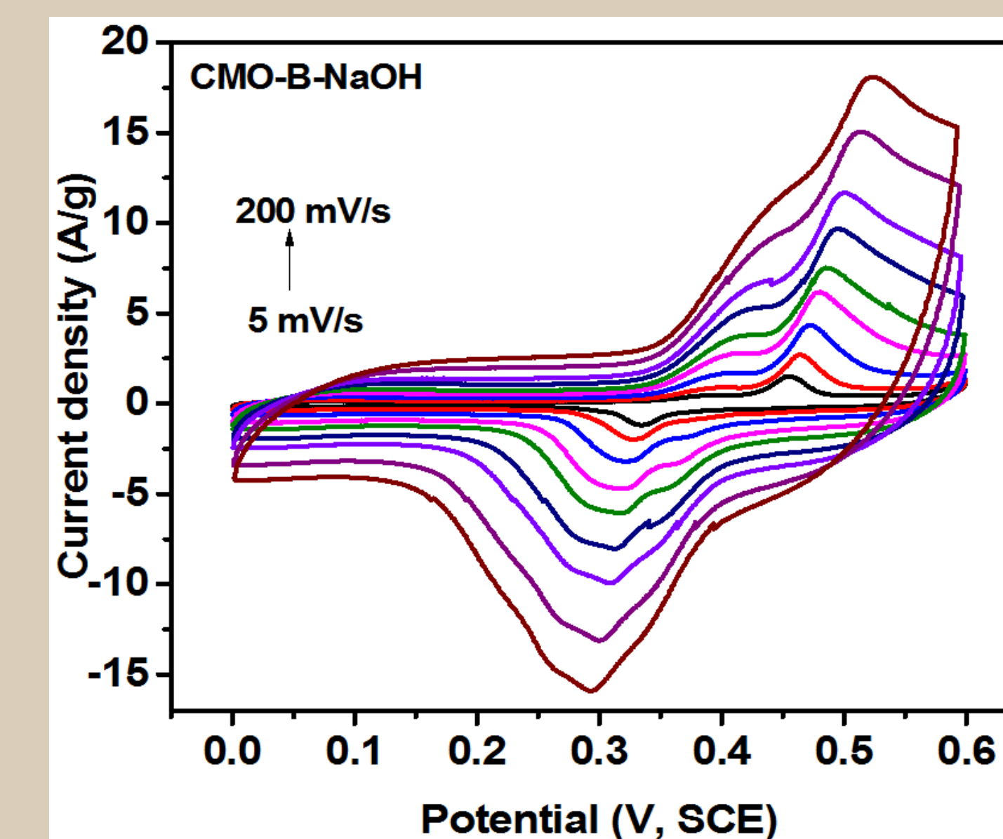
Cyclic voltammograms of CMO-B (heating rate 3^\circ \text{C}/\text{min} ) sample at various scan rates in 3 M NaOH electrolyte.
