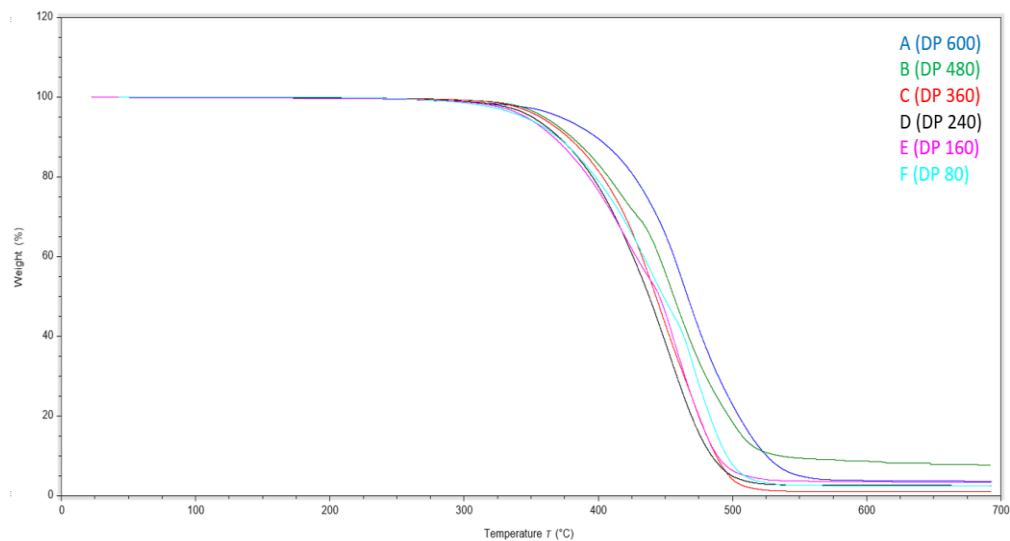
Figure 2.5: TGA traces of 5% MeTfpS-Containing Terpolysiloxanes with Varying DPs from 80 to 600.
