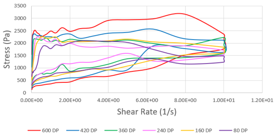
Figure 6.36: Steady Shear Rheology of 5% MeTfpS-Containing Terpolysiloxane
