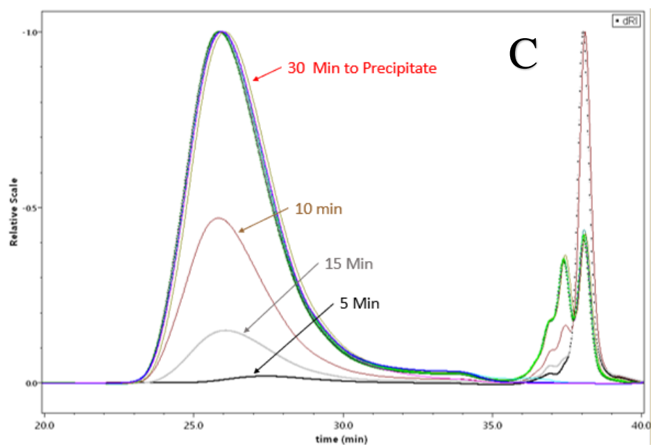
Figure 6.2: SEC Monitoring of the Synthesis of 5% MeTfpS-Containing Terpolysiloxane C Having Targeted DP of 360
