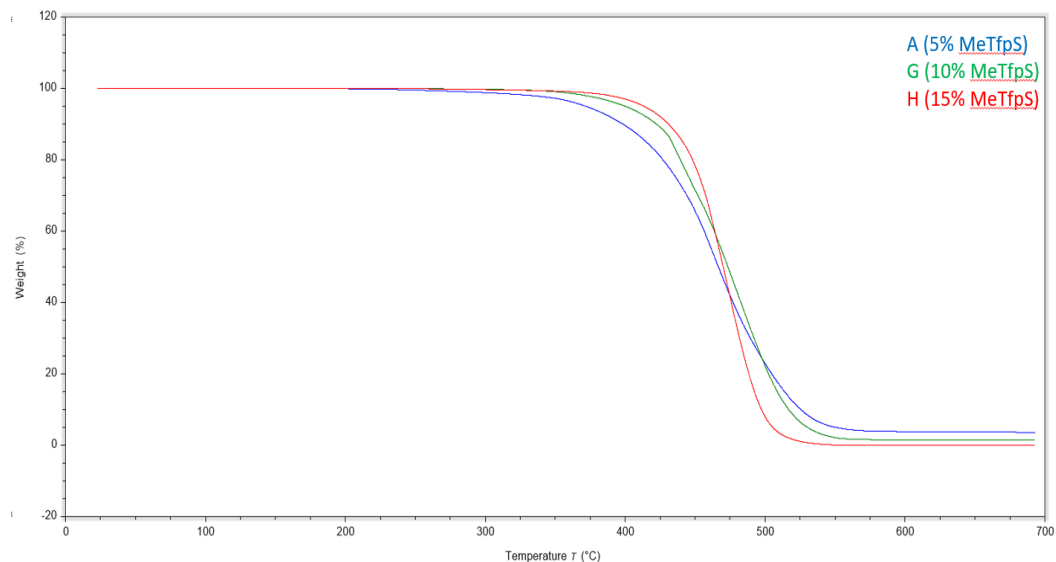
Figure 2.6: TGA traces of 5, 10, and 15% MeTfpS-Containing Terpolysiloxanes with DP of 600.
