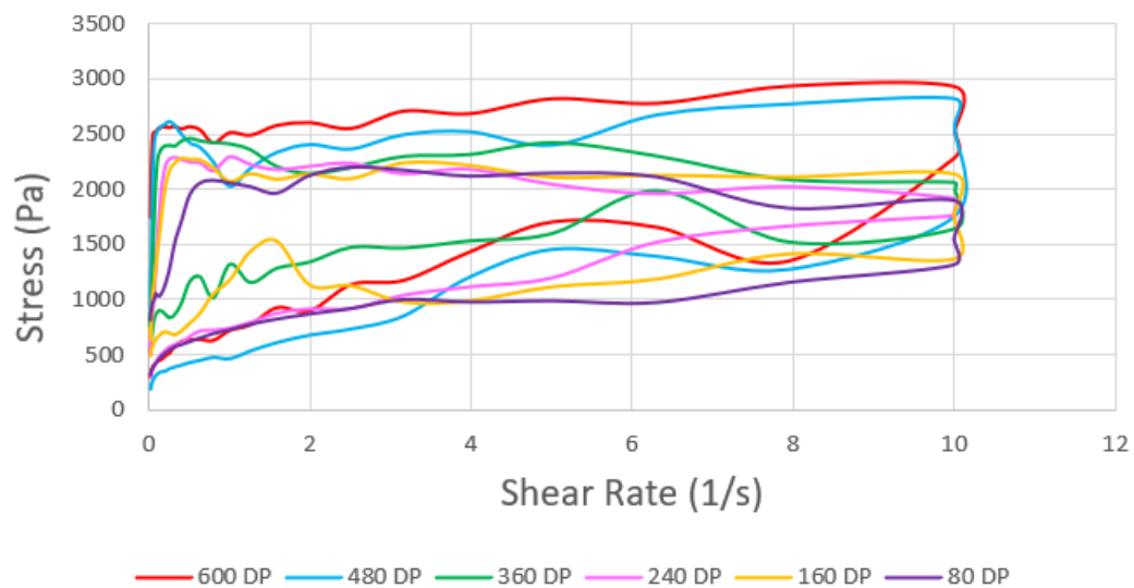
Figure 6.33: Steady Shear Rheology of 5% MeTfpS-Containing Terpolysiloxane
