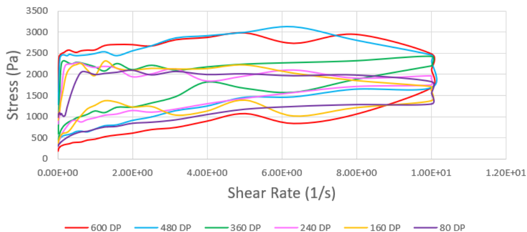
Figure 6.34: Steady Shear Rheology of 5% MeTfpS-Containing Terpolysiloxane Pastes with Varying Degrees of Polymerization from 80 to 600, Month Five
