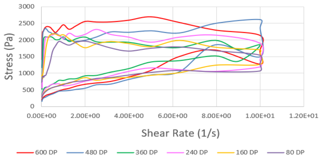
Figure 6.37: Steady Shear Rheology of 5% MeTfpS-Containing Terpolysiloxane
