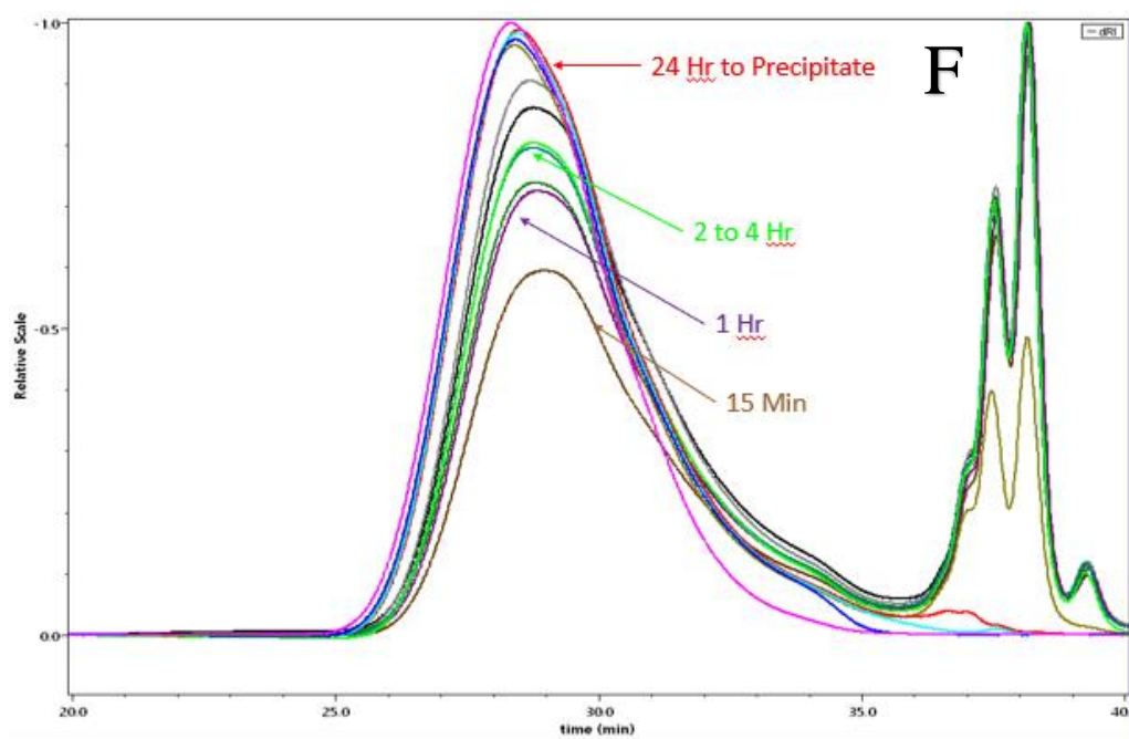
Figure 6.5: SEC Monitoring of the Synthesis of 5% MeTfpS-Containing Terpolysiloxane F Having Targeted DP of 80
