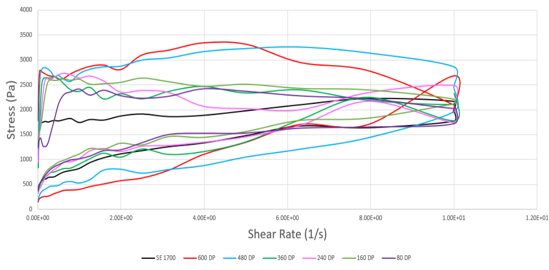
Figure 6.30: Steady Shear Rheology of 5% MeTfpS-Containing Terpolysiloxane Pastes with Varying Degrees of Polymerization from 80 to 600, Month One
