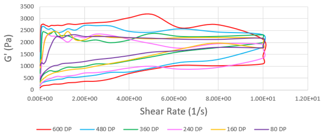
Figure 6.32: Steady Shear Rheology of 5% MeTfpS-Containing Terpolysiloxane
