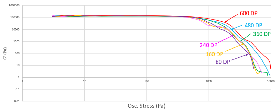
Figure 6.19: Oscillatory Rheology of 5% MeTfpS-Containing Terpolysiloxane Pastes with Varying Degrees of Polymerization from 80 to 600, Month Four
