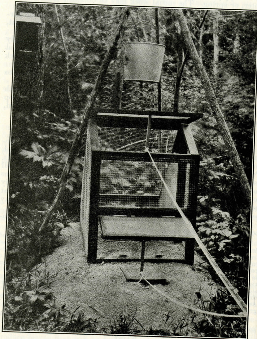
FIGURE 60.—Combination trap baited with water, showing a method of suspending the storage reservoir over the trap. The basin is almost concealed by the lower door. (Photograph by Karl Christofferson)
