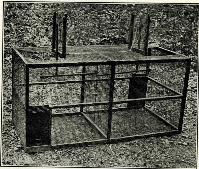
FIGURE 27.—Chardonneret trap—an excellent top-opening type. Pressure of the door spring, transmitted through the centerpiece, holds the triggers in place against the vertical rod between the cells. A bird dropping onto the trigger dislodges it and allows the spring to close the door.
