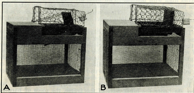
FIGURE 17.—Resetting trap. A. Tilting chamber up; B, tilting chamber down. The bait pans do not show clearly, but they are located on either side of the moving chamber. The door for removing captured birds shows faintly in the lower right-hand corner. (Photos by William I. Lyon)
