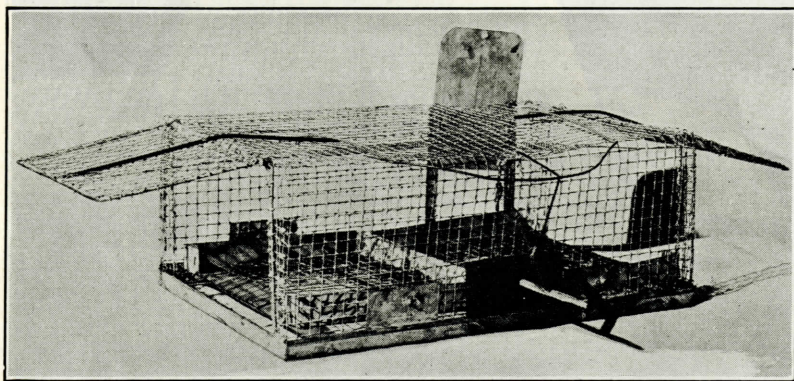
FIGURE 25.—Two-door trap (automatic; Everett type). The trigger wires do not overlap, as in the Higgins type; and are held in place by a wire ball, which in turn is held by the trigger cord connecting to the figure-4 release. This last is operated by the movement of the pivoted treadles. The sliding door for the removal of captured birds is shown open. (Photograph by E. A. Everett)
