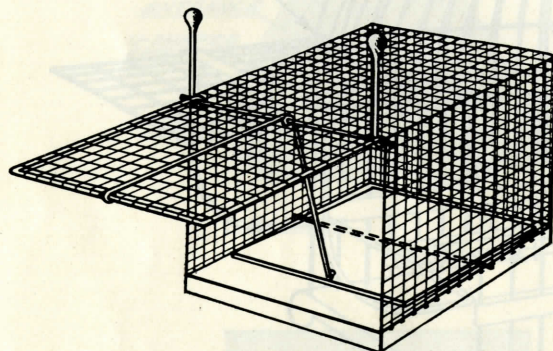
FIGURE 22.—False-bottom trap. The moving bottom, or treadle, is pivoted in two meshes of the sides. It engages with the trigger attached to the door, which is closed and held shut by the lead weights.
