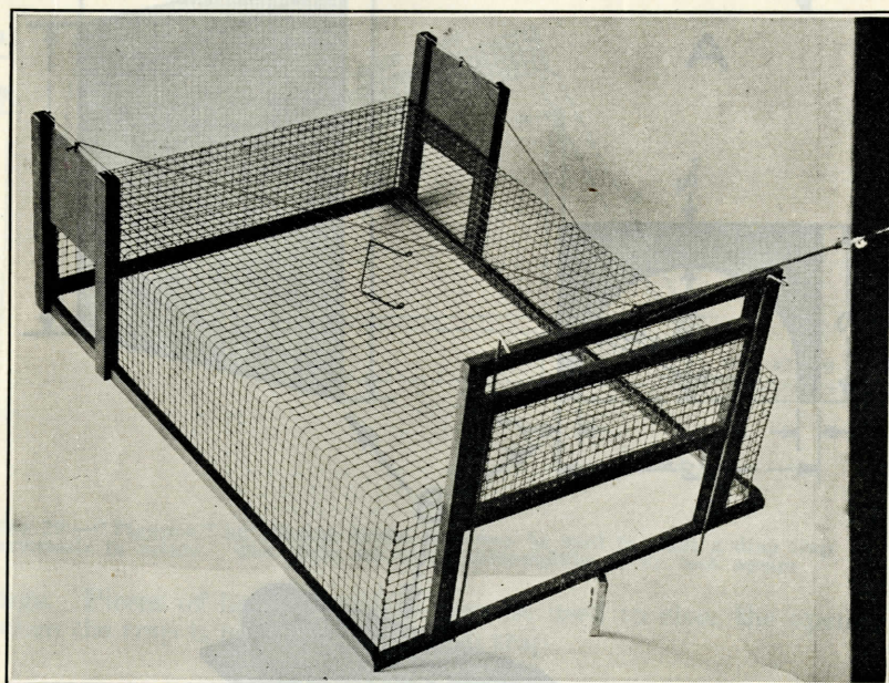
FIGURE 12.—Triplex trap. The cords from all three doors come together at the ring. The vertical wire rods hold the front door in place.
