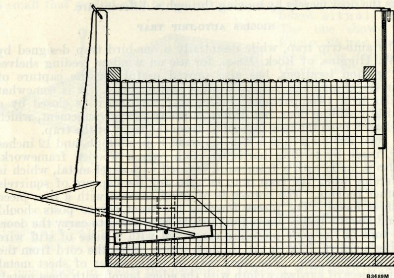
FIGURE 23.—Details of Higgins auto-trip trap, showing bait pan and the figure-4 device used to release the door
