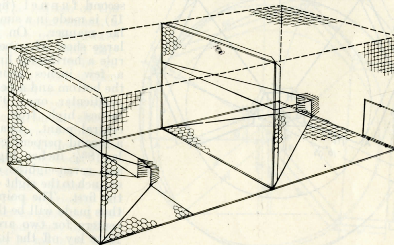
FIGURE 13.—Details of construction of modified Government sparrow trap. Relative position of funnels and door is shown.
