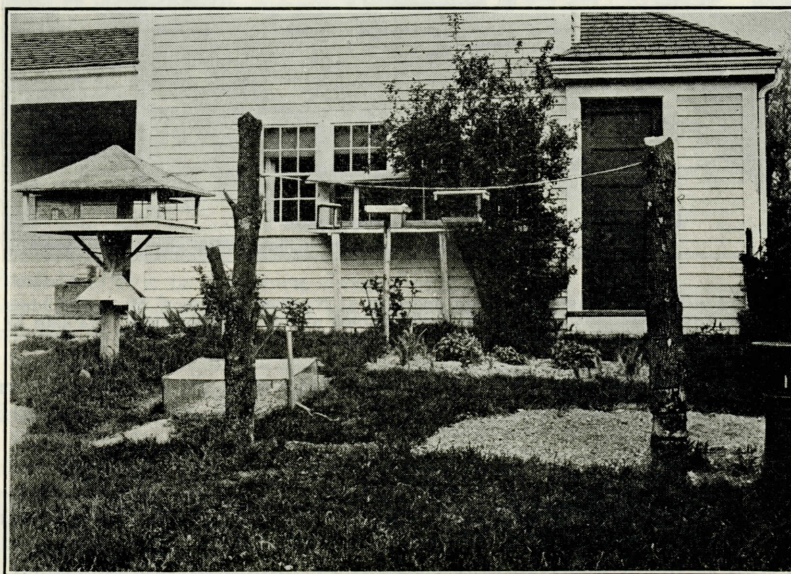
FIGURE 3.—An efficient banding and feeding station in a small yard at Cohasset, Mass. From left to right, the equipment is: A "pagoda" weatherproof feeder, with zinc cat guard; on the ground, a collapsible drop trap (see fig. 8), operated from the window; on the window ledge, a 5-foot feeding shelf with a small trap; in front of the window, a feeding trap on a 4-foot pole; suspended between the two posts, another feeder hung on a wire; and at the extreme right, a 14-inch flowerpot saucer bath on a standard about 3 feet high. (Photo by the station operator, Charles L. Whittle)
