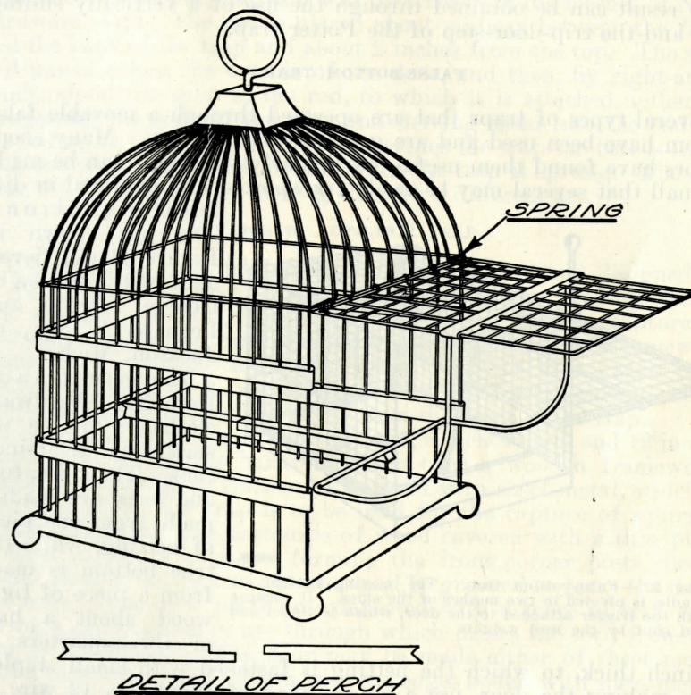
FIGURE 21.—Canary-cage trap. Simple in construction and admirably suited for window-feeding shelves
