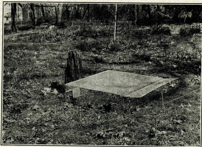
FIGURE 8.—Beginner's flat trap. An excellent type for work with ground-feeding birds, which are rarely, if ever, injured by its operation
