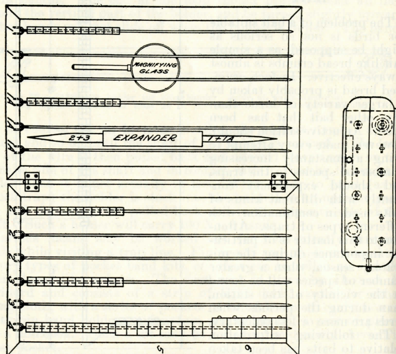
FIGURE 59.—Pocket band kit. Light frames made from wood half an inch square and backed with light sole leather or stout cardboard are hinged together to make a book-like case. The bands are carried on galvanized-wire needles, pointed at one end and with small rings in the other, by means of which they are attached loosely to the frames by small staples
