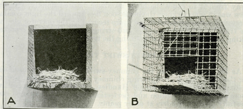
FIGURE 40.—Baldwin nesting box and nest trap. A, The box occupied by a robin's nest; B, the box with the trap in place and the door open, showing the outside platform
