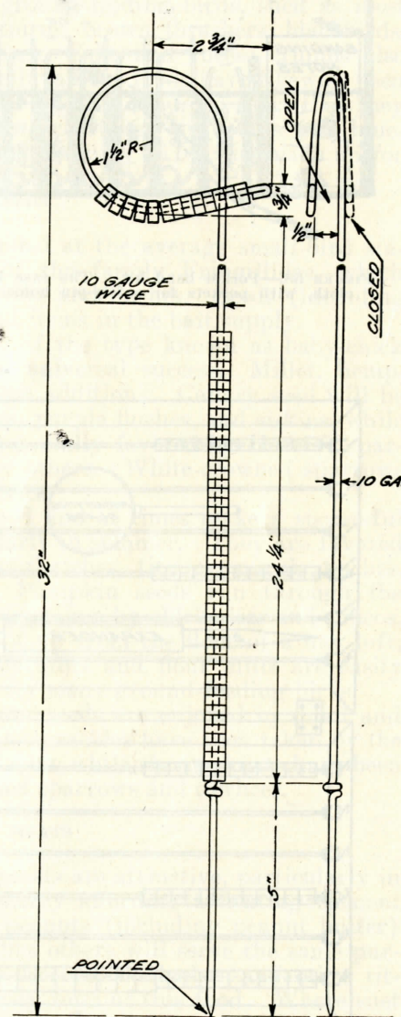
FIGURE 57.—Holder for large bands
