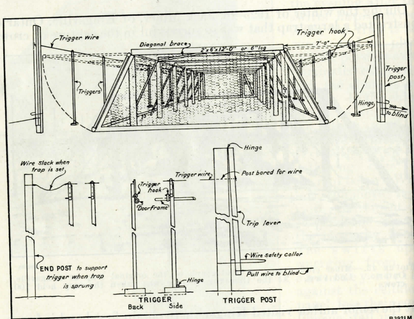
FIGURE 44.—Details of Miner crow trap. The trap is built on heavy posts, with scantlings, ordinary 2-inch-mesh poultry wire, and ½-inch iron-pipe doors. Traps of this same type have been successfully used to capture geese for banding
