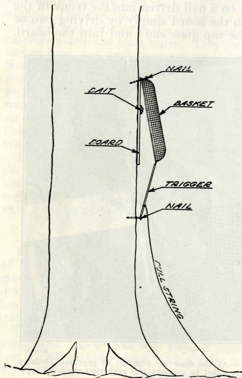
FIGURE 30.—Basket trap. A wire letter basket is attached loosely by staples to a board that may be hung on a tree trunk. A pull string is attached to a light stick, one end of which rests on a nail driven into the tree, while the other end props the lower end of the basket away from the board.
