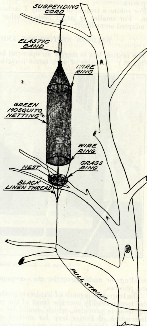
FIGURE 38.—Details of Duer nest trap
