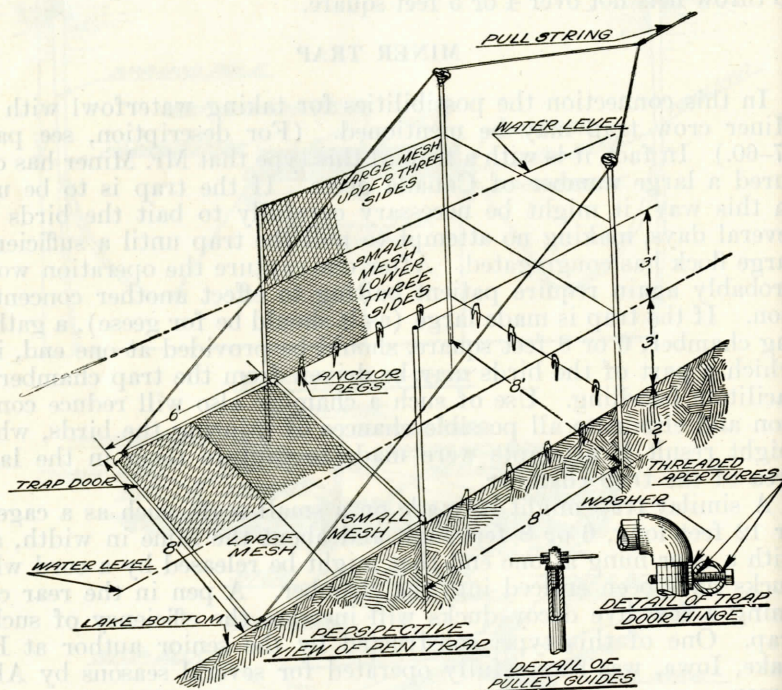
FIGURE 52.—Details of pen trap for diving ducks
