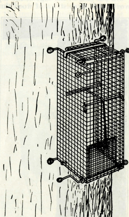
FIGURE 31.—Baldwin woodpecker trap. A bird entering the trap from below climbs up the tree trunk to get the bait placed just above the cross-arms of the trigger. These are naturally touched and lifted enough to release the lower door from the W-shaped hook on the lower end of the trigger.
