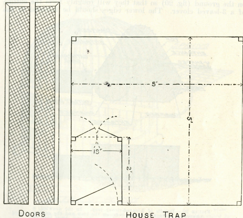
FIGURE 19.—Ground plan of house trap shown in Figure 18. The drawing shows the vestibule and the correct position of doors when the trap is set
