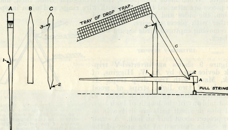
FIGURE 10.—“Figure-4,” an efficient device that may be used to make a drop trap automatic in action. The sticks are about three-eighths of an inch square
