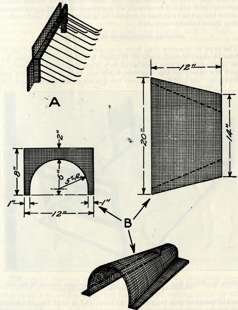
FIGURE 11.—Automatic attachments for drop traps. A, Attachment made by fastening to a hardware cloth frame a series of guard wires that will project into the trap chamber and that can be raised or lowered as desired (Northeastern Bird Banding Association type); B, half-funnel attachment, showing shape of the hardware-cloth arch to which it is attached, pattern for cutting the half-funnel, and the finished passage. (After G. D. Sprot)
