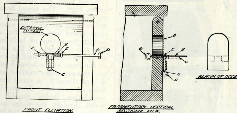
FIGURE 34.—Details of construction of nest-box trap
