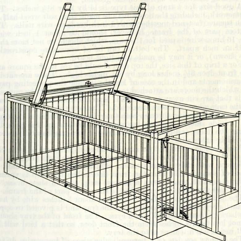
FIGURE 26.—Lurvey combination trap. The top door is held open by the trigger post rising perpendicularly from the middle point of one side of a pivoted bait tray engaging with a trigger wire attached to the door. The secondary trigger wire (shown as a dotted line) is projected by opening the top door, so that the trigger hook on the front door may be engaged with it. This drawing shows the way in which the doors are pivoted, the springs attached, and also the figure-4 catch to lock the front door.
