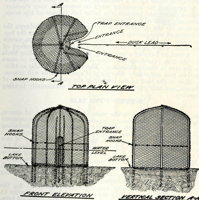
FIGURE 48.—Details of waterlily-leaf trap. An apron of netting extending onto the bottom from the sides prevents captured birds from diving under the side walls and escaping
