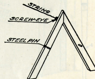
FIGURE 9.—Inverted-V device for use with trap drop traps. Two small nails or steel pins support the trap through the meshes of the netting. The pull string is attached to a screw eye at the apex on the other side
