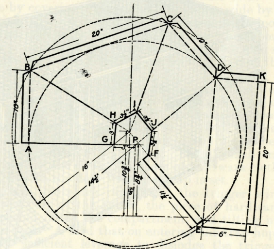
FIGURE 15.—Pattern for second funnel of trap shown in Figure 13
