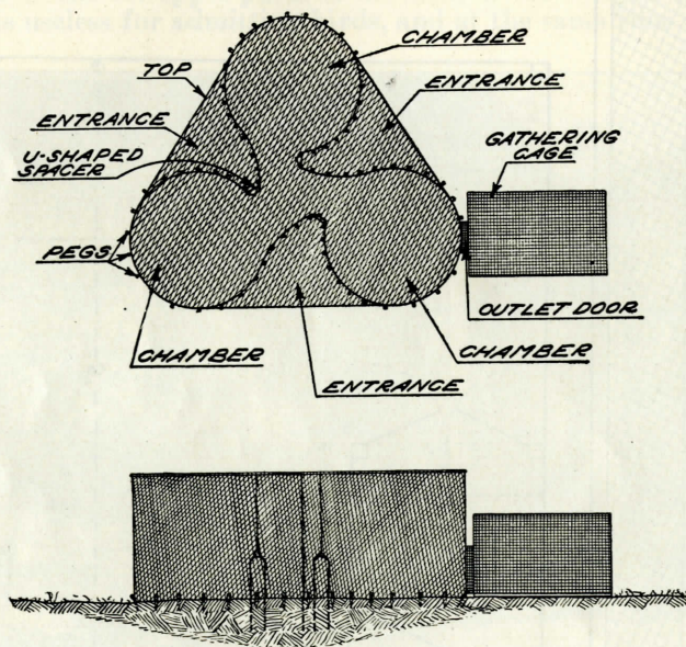
FIGURE 20.—Details of 3-leaved-clover trap. In the drawing, a connecting passage is shown between the trap and the gathering cage, but this is rarely needed, as the two doors may be placed in actual contact
