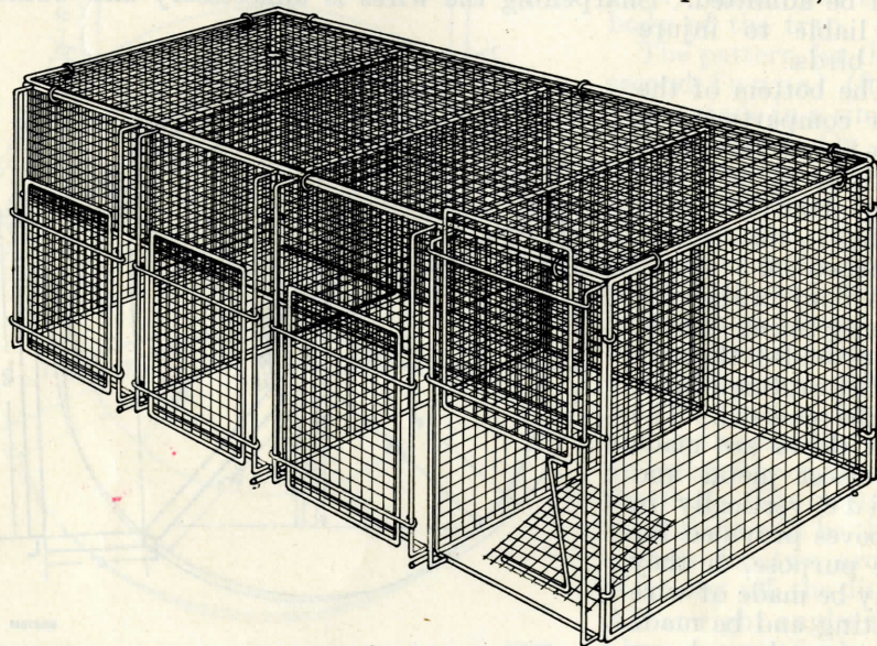
FIGURE 16.—Details of 4-celled Potter trap, showing the projecting door frames, or slides, and the manner in which the doors are attached to them
