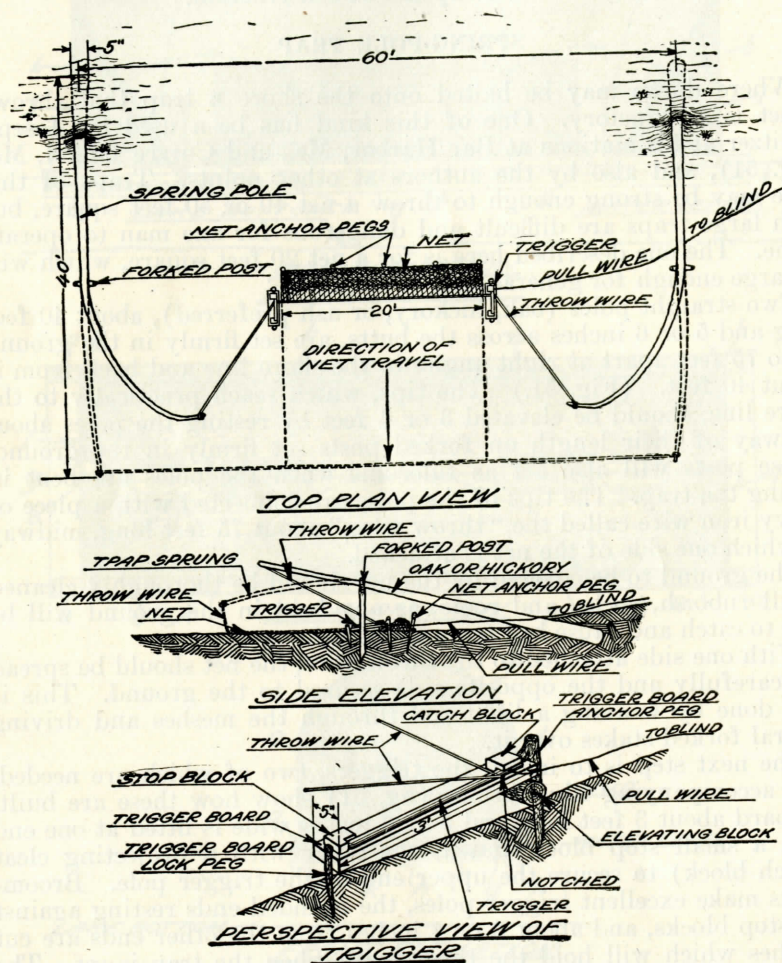
FIGURE 51.—Details of spring-pole trap with net 20 feet square
