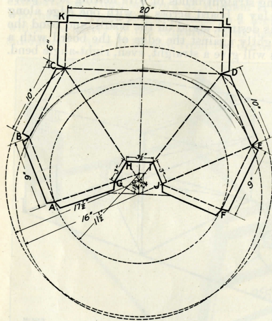
FIGURE 14.—Pattern for first funnel of trap shown in Figure 13
