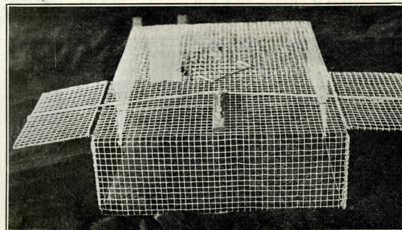
FIGURE 24.—Two-door trap (Higgins type). The two doors are connected on the inside by a light spring (or an elastic band), and when set, the trigger wires lie on top of the cage, overlapping about an inch, and are held in place by the short trigger, which is jerked out when the trap is sprung. (Photograph by A. W. Higgins)
