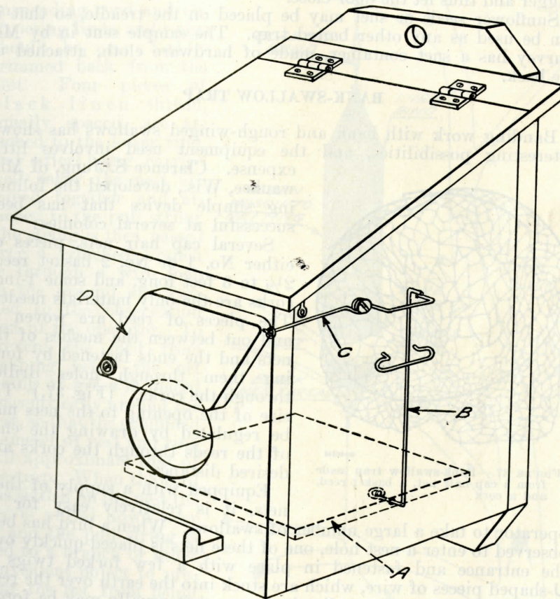
FIGURE 36.—Lurvey trap No. 3. A bird entering the box through the hole provided hops onto the tilting treadle A, which moves the lever B, disengaging the pivoted trigger C, and allowing the shutter D to descend of its own weight and close the opening.
