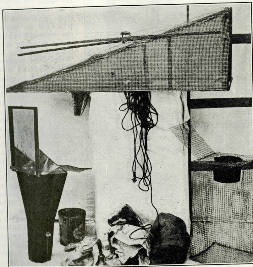
FIGURE 41.—Chimney-swift trap. Above is the trap chamber, made of light poplar strips, the sides covered with muslin and the top with \frac{1}{2} -inch-mesh twine netting, and with flaps of pigeon wire for attaching to chimney; at the left is a celluloid panel attached to the chute; in the lower right-hand corner is a gathering cage with safety door raised; and in the center are various implements, a pail, bell, burlap sack, roll of newspaper, etc., that can be lowered into the chimney to start the birds. (Photograph by Charles O. Handley)
