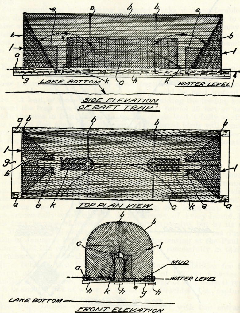
FIGURE 50.—Details of raft trap. The framework of galvanized-iron pipe ( b ) is secured to the raft made by bolting planks ( g , h ) to two 40-foot logs ( a ). The funnels ( l ) terminate in entrances that may be closed by doors ( k ) hinged to the raft or platform. Short deflecting wings ( e ) will turn captured birds away from the entrance. A semicircular pen ( c ) confines a few live decoys
