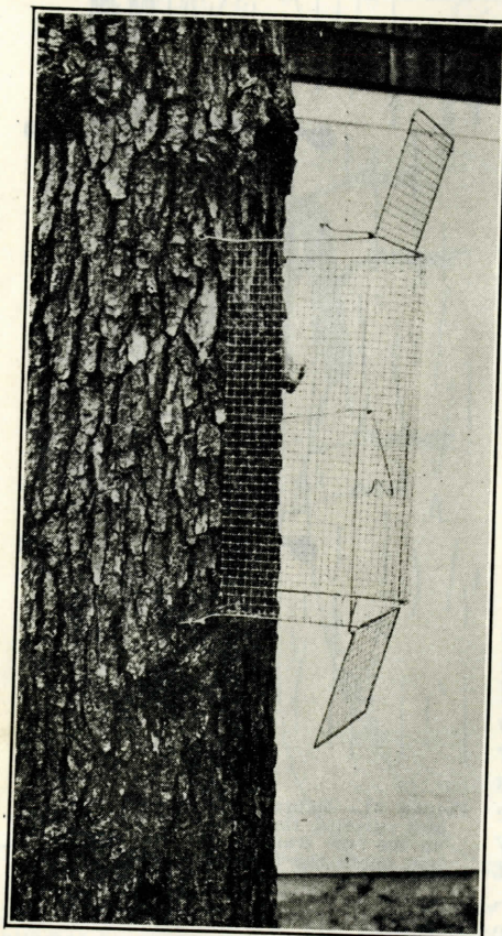
FIGURE 32.—Baldwin woodpecker trap used with a pull string. The cranks on both doors are connected so that the doors will close simultaneously
