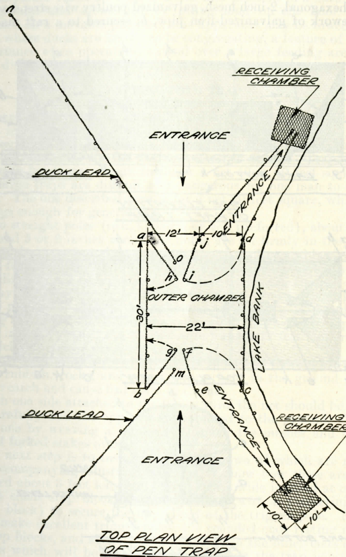
FIGURE 49.—Details of McIlhenny pen trap. The large outer chamber (a, b, c, d) is provided with large funnels (a, h, i, j and b, g, f, e), which are approached by leads (l, m and n, o). Funnel-shaped passages lead from the outer chamber to the receiving chambers, which are entered by funnels 4 to 6 inches wide. When the trap is not in operation, entrance to the receiving chambers is blocked by moving the funnel wings (i, j and e, f) to the positions d, j and c, e, the opposite wings (a, h and b, g) being moved against the front of the outer chamber.
