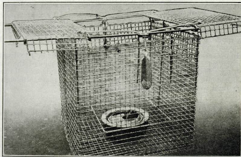
FIGURE 28.—Michener water trap. When a bird touches the wire treadle around the drinking vessel, the trigger is released from the door to the right. This permits lead weights to close both doors. (Photograph by Harold Michener)
